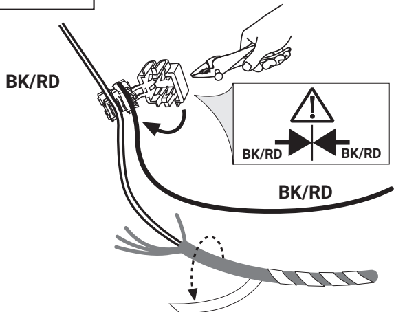
Network control unit connector C
